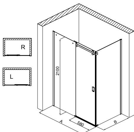
Muna Eckversion / Corner version
