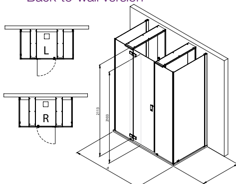
Thasos for two Vorwandversion / Back-to-wall version
