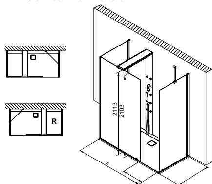
Thasos Vorwandversion / Back-to-wall version
