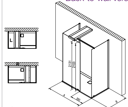
Ciela Vorwandversion / Back-to-wall version
