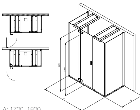
Ciela for two Vorwandversion / Back-to-wall version
