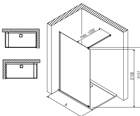
One&One Eckversion / Corner version
