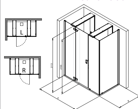
Thasos for two Eckversion / Corner version
