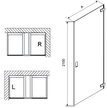
Ciela Tür / Shower door
