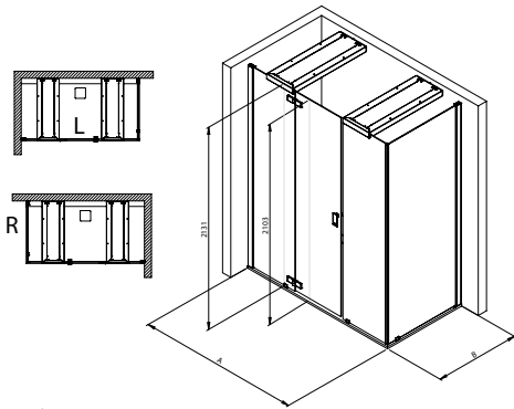
Ciela for two Eckversion / Corner version
