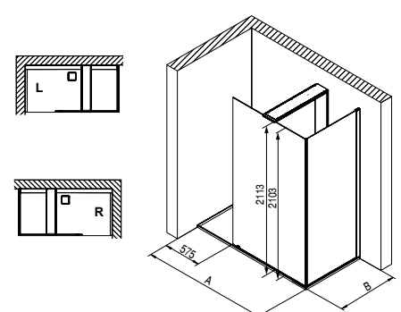
Thasos Eckversion / Corner version
