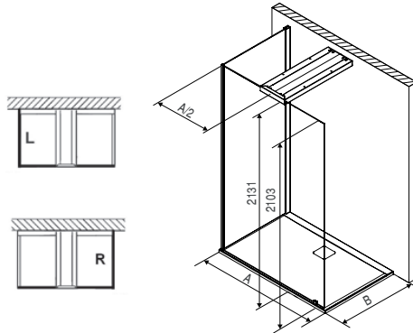
Ciela Vorwandversion B / Back-to-wall version B
