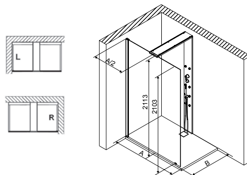
Thasos Eckversion B / Corner version B
