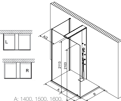
Thasos Vorwandversion B / Back-to-wall version B
